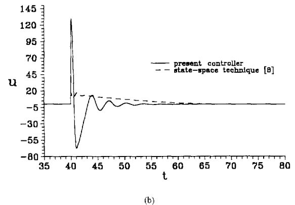
Fig. 5. Time responses of (a) the x -output for two different controllers and (b) the control input, u is activated at time t = 40 , for the case of control the state to the new fixed point on the equilibrium manifold.
