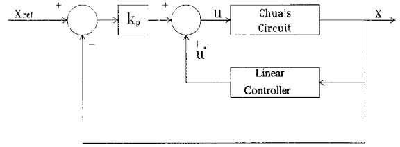
Fig. 1. Block diagram representation of the controlled system.
