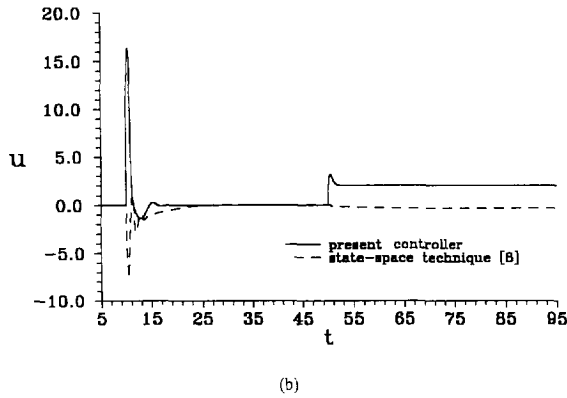
Fig. 6. Time responses of (a) the x -output for two different controllers and (b) the control input, u is activated at time t = 10 , for the case of control input is changed from \sqrt{0.5} to 1 at time t = 50 .
