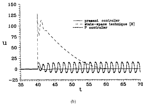
Fig. 4. Time responses of (a) the x -output for three different controllers and (b) the control input, u is activated at time t = 40 , for the case of control the state to the original equilibrium point.
